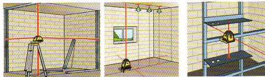
LEVELING, SQUARING, PLUMBING
