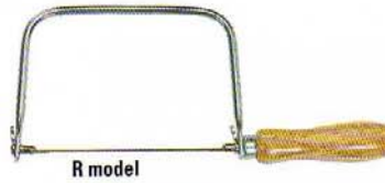
R model
